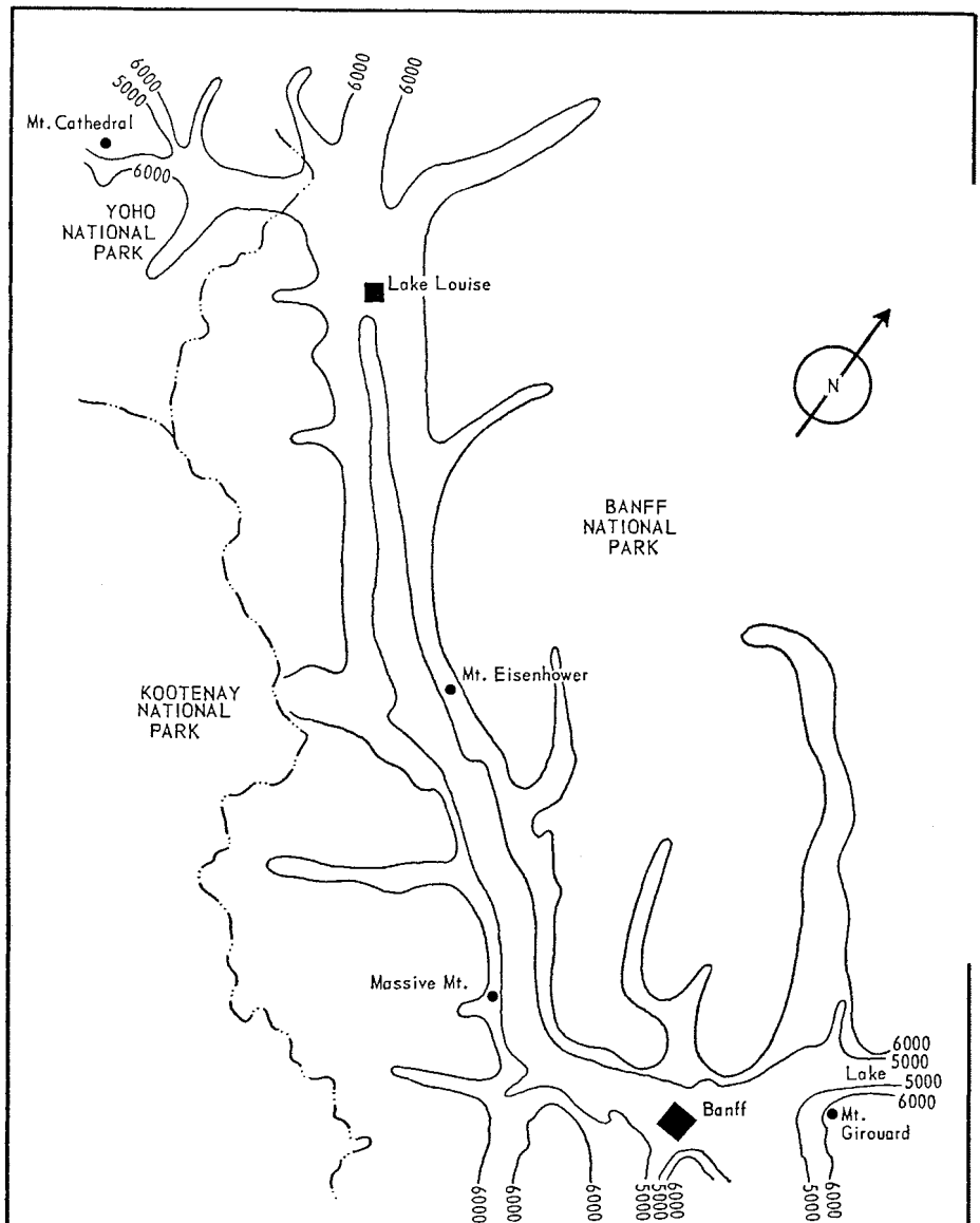
FIG. 1. Schematic illustration of the four sampling areas, the two climatological stations, and the 5000- and 6000-ft contour lines.
